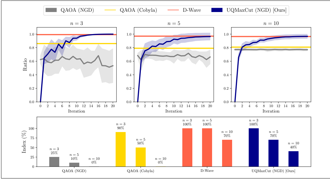
Figure 4.3.2: Experimental comparison of the proposed Universal Quantum Max-Cut (UQMaxCut) algorithm with QAOA and D-Wave. Results are shown for fully-connected graphs of n = 3, 5 , and 10 nodes with strictly positive edge weights, and are averaged over 20 random graph instances for each n . (Top row) Approximation ratio (larger is better). The lines represent the averaged ratios over the 20 instances and the shaded areas indicate the standard deviations. (Bottom row) The approximation index, i.e., the percentage of instances where a global solution is found. All gate-based methods (QAOA and UQMaxCut) less frequently return a global solution for larger n . Yet, in contrast to QAOA, D-Wave and the proposed UQMaxCut also consistently return very good approximate solutions, i.e., points whose function values are very close to the global minimal function value.
