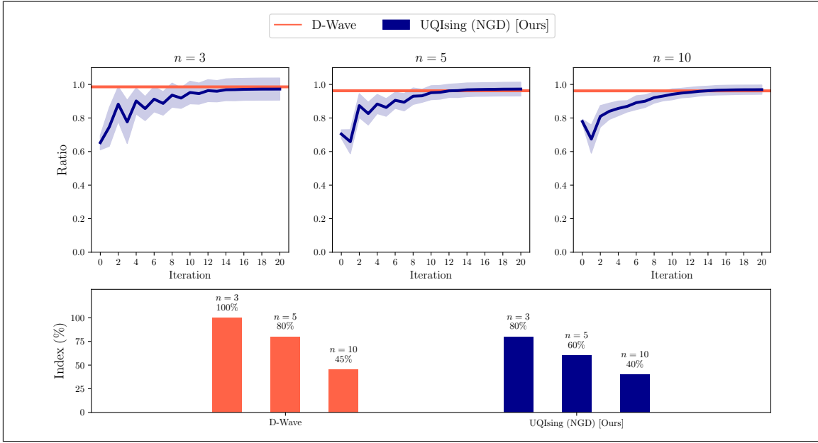
Figure 4.3.3: Experimental comparison of the proposed Universal Quantum Ising Model (UQIsing) algorithm with D-Wave. Results are shown for fully-connected graphs of n = 3, 5 , and 10 nodes with strictly positive edge weights. They are averaged over 20 random graph instances for each n . (Top row) The approximation ratio. The lines represent the averaged ratios over the 20 instances and the shaded areas indicate the standard deviations. (Bottom row) The approximation index, i.e., the percentage of instances where a global solution is found. Our method can compete with D-Wave solvers in predicting approximate solutions and finding the global minimum for moderate n .
