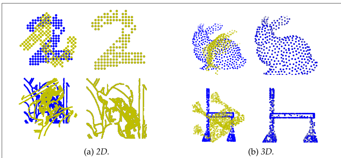
Figure 1.2.4: Iterative quantum approach for transformation estimation. (a) Registration results on 2D point sets (MNIST [21] and Lena [22]). (b) Registration results on 3D point sets (Stanford bunny [23] and completion3D [24]). Blue points represent reference points and olive points represent template points. The initial alignment is shown on the left and the result of the registration on the right. See Chapter 6 for a full discussion.
