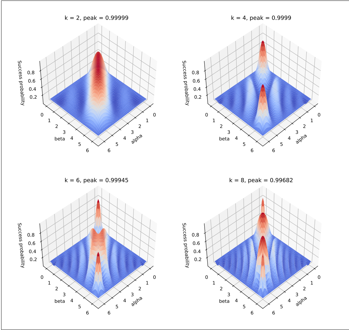
Figure 5.1.1: Phase matching in quantum search. The initial vector of the algorithm is a state vector |\psi_0\rangle = \sqrt{a} |\eta_+\rangle + \sqrt{1-a} |\eta_-\rangle with a = 1/10 . At each iteration, the oracle marks the solution with phase \alpha , while the diffusion operator marks the initial state with phase \beta . (From left to right, top to bottom) On the vertical axis is the probability of measuring a solution, |\eta_+\rangle , after k iterations. We see that the success probability peaks on the diagonal, when \alpha and \beta satisfy the phase matching condition.
