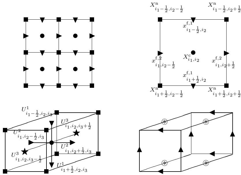
Figure 3. Staggered grids, nodal \blacksquare , cell centered \bullet , face-staggered grids ( \blacktriangledown in the x_1 -, \blacktriangleright in the x_2 - and \blackstar in the x_3 -direction), and edge-staggered grids ( \blacktriangle in the x_1 -, \blacktriangleleft in the x_2 - and \otimes in the x_3 -direction). Top left: d = 2 , four pixels, top right: d = 2 pixel (i_1, i_2) with grids, bottom left: d = 3 , voxel (i_1, i_2, i_3) with face-staggered grids and positions of U^1, U^2, U^3 , bottom right: d = 3 , edge-staggered grids.
